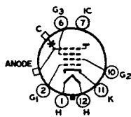
12C ANODE - G_4 + C_1 FOCUSING ELECTRODE - G_3
