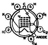
81P ANODE - G_3 + G_5 + C_1 FOCUSING ELECTRODE - G_4
