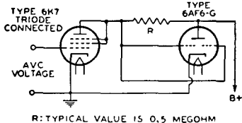
Fig. 111—Indicating circuit using 6AF6G electron-ray tube and external dc amplifier.
