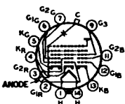
ULTRON = G_4 + G_5 + Cl FOCUSING ELECTRODE = G_3
