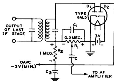
Fig. 62—Delayed avc (davc) circuit.
