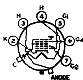
77A ANODE - G_3 + G_4 + C_1 FOCUSING ELECTRODE - G_4
