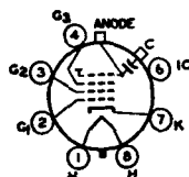
81R ANODE - G_4 + C_1 FOCUSING ELECTRODE - G_3
