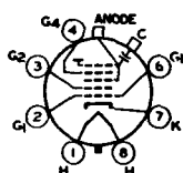
81E ANODE - G_3 + G_5 + C_1 FOCUSING ELECTRODE - G_4
