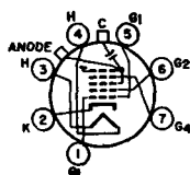
7GR ANODE - G_3 + G_5 + C_1 FOCUSING ELECTRODE - G_4
