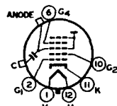
12L ANODE - G_3 + G_5 + C_1 FOCUSING ELECTRODE - G_4
