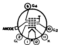
ANODE = G_3 + G_5 + Cl FOCUSING ELECTRODE = G_4
