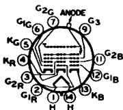
ANODE = G_4 + G_5 + Cl + R FOCUSING ELECTRODE = G_3
