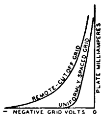
Fig. 38—Plate-current curves for triodes having remote-cutoff and uniformly spaced grids.
