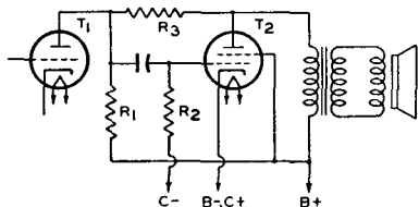
Fig. 50—Resistance-coupled stages using feedback resistor.
