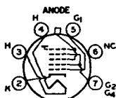
77G ANODE - G_3 + G_5 + C_1 AUTOMATIC FOCUSING
