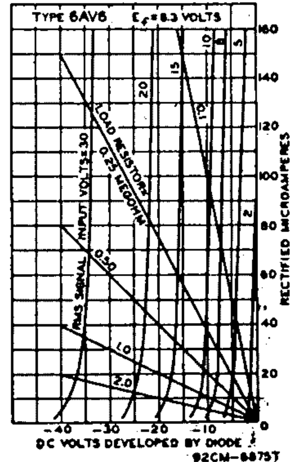
AVERAGE DIODE CHARACTERISTICS HALF-WAVE RECTIFICATION-SINGLE DIODE UNIT
