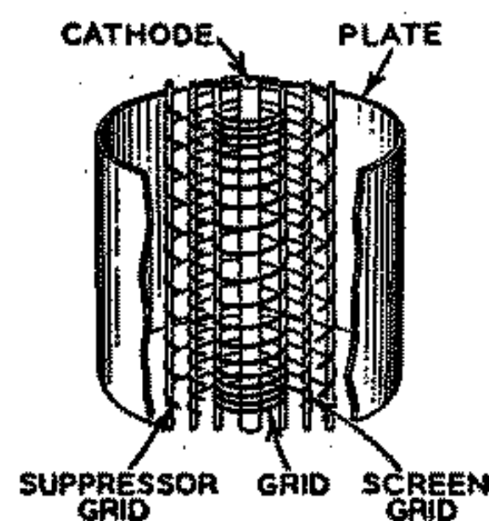
Fig. 37—Structure of remote-cutoff grid.
