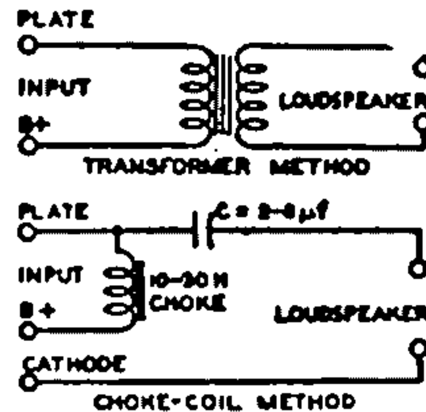
Fig. 123—Typical output-coupling devices.
