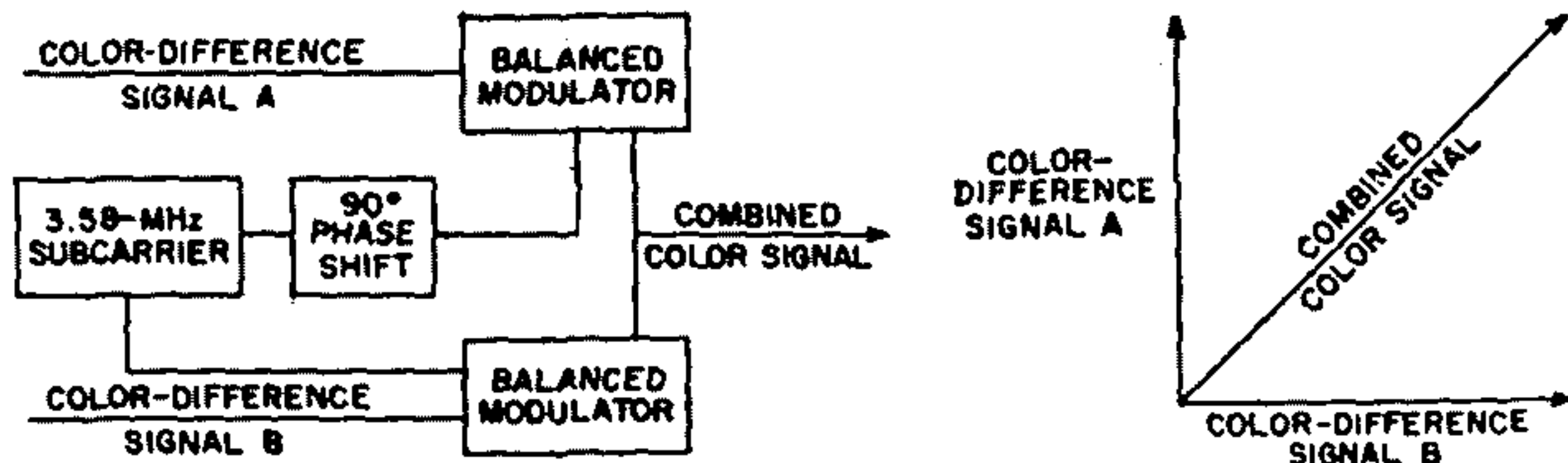
Fig. 93—Formation of combined color signal for transmission.
