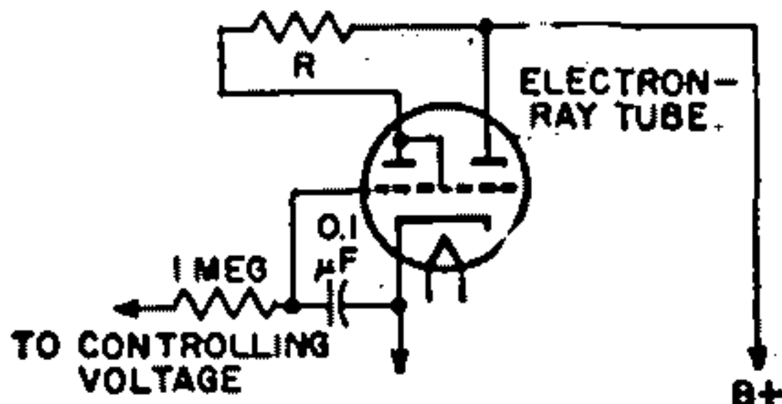
Fig. 110—Indicating circuit using an electron-ray tube.
